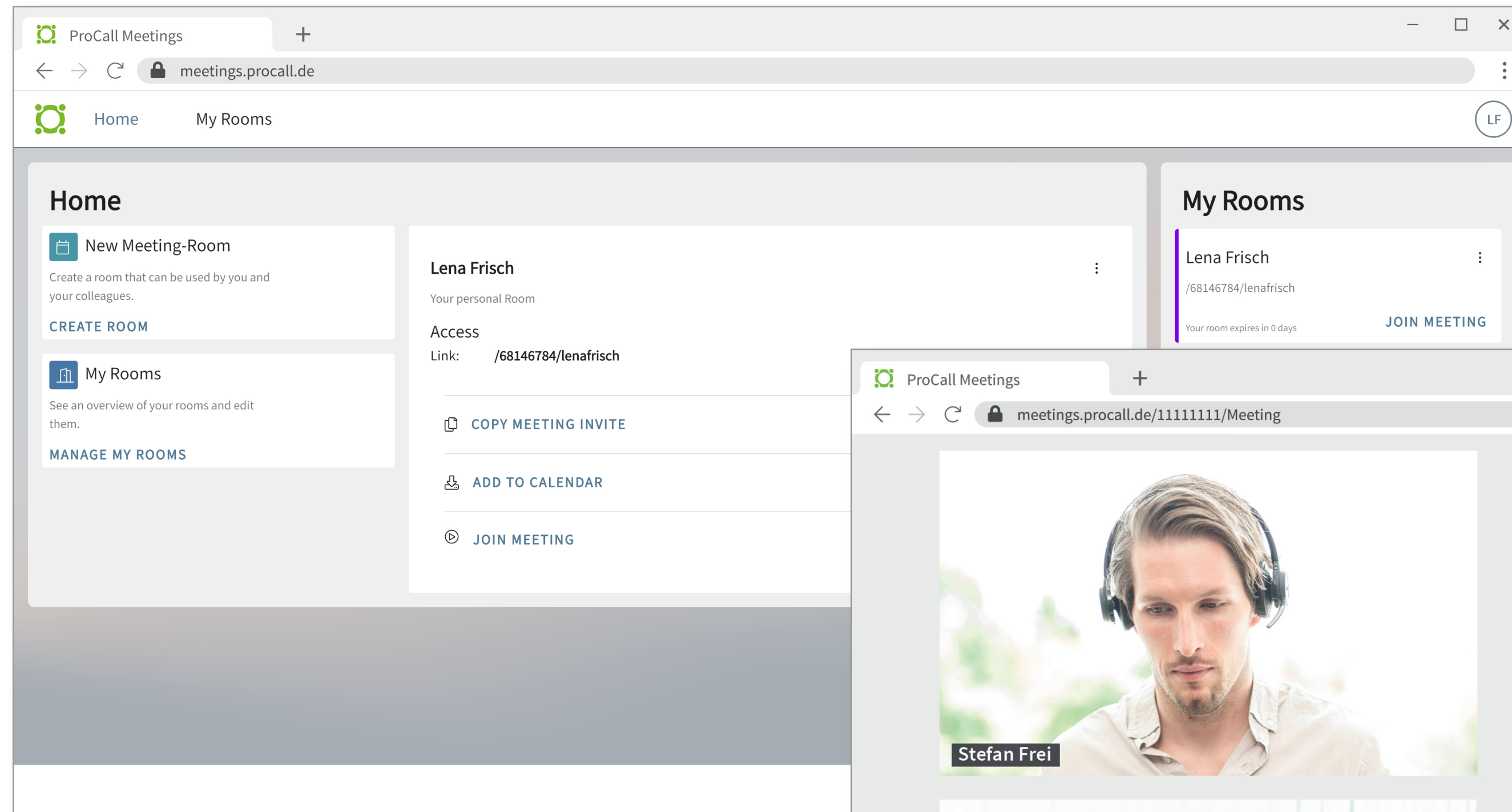
Personal dashboard
