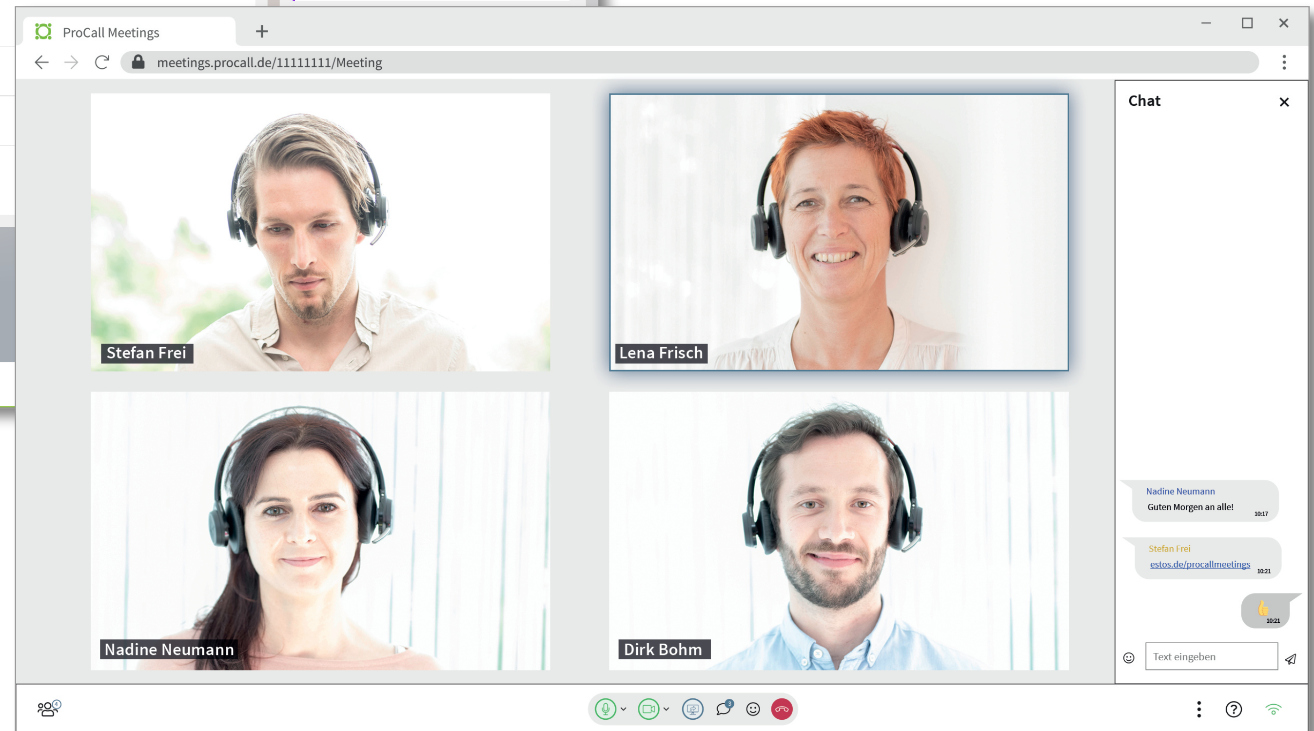
Video conference
